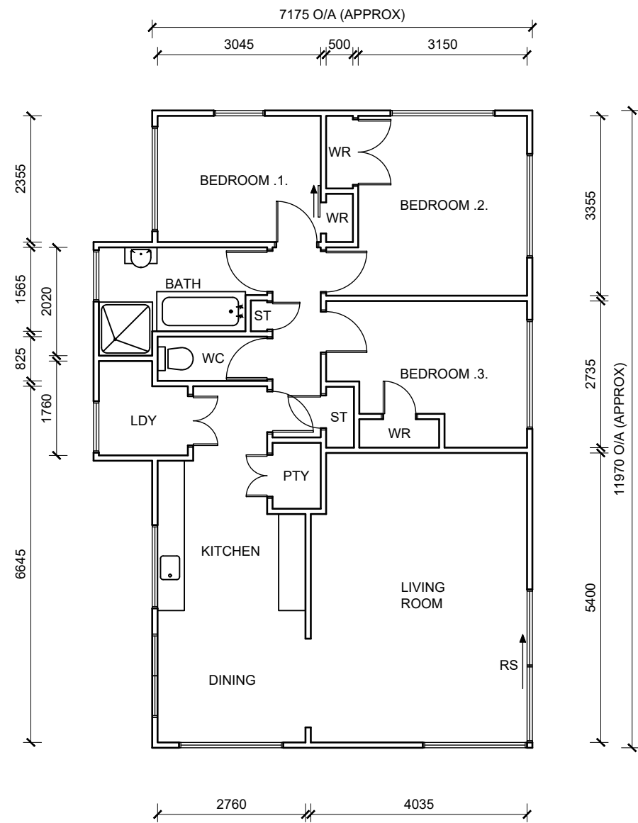
EXISTING FLOOR PLAN SCALE 1:100 @ A3
